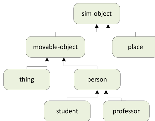
Figure 10.2. Inheritance Hierarchy.
