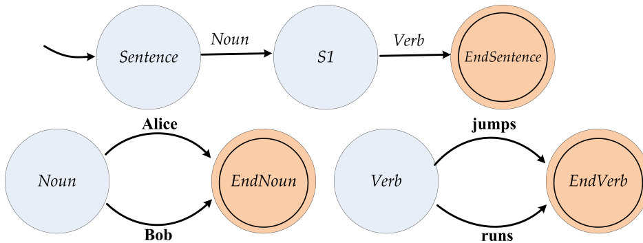
Figure 2.4. Recursive transition network with subnetworks.
