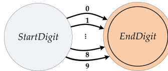
Figure 2.11. Converting the Digit productions to an RTN.
