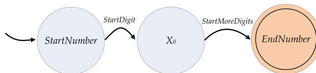
Figure 2.9. Converting the Number productions to an RTN.
