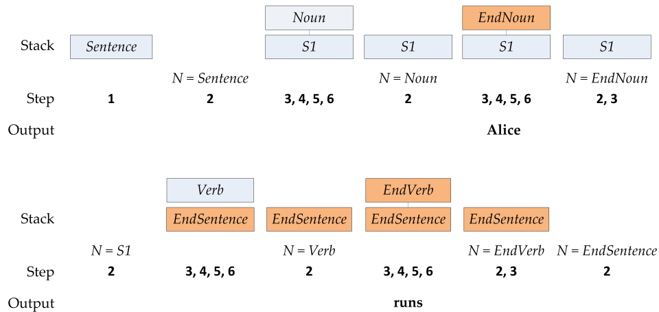
Figure 2.6. RTN generating “Alice runs”.
