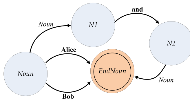
Figure 2.5. Alternate Noun subnetwork.
