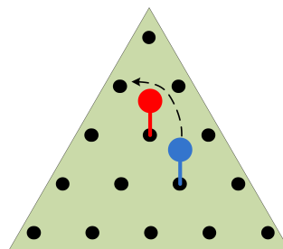
Figure 5.1. Pegboard Puzzle.
