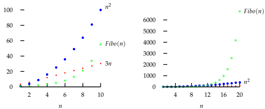
Figure 7.3. Orders of Growth.
