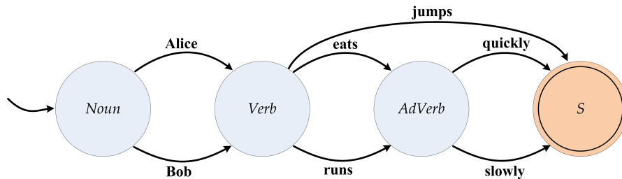
Figure 2.3. RTN for Exercise 2.6.
