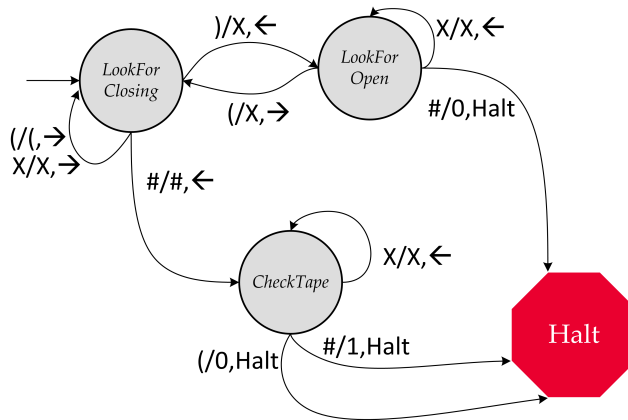
Figure 6.8. Checking parentheses Turing Machine.
