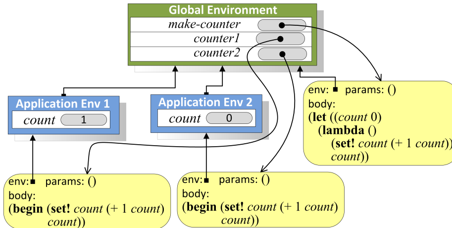
Figure 10.1. Environment produced by evaluating:
