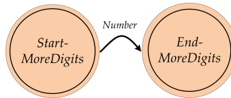
Figure 2.10. Converting the MoreDigits productions to an RTN.
