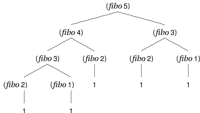
Figure 7.1. Evaluation of fibo procedure.
