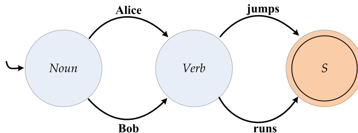
Figure 2.1. Simple recursive transition network.
