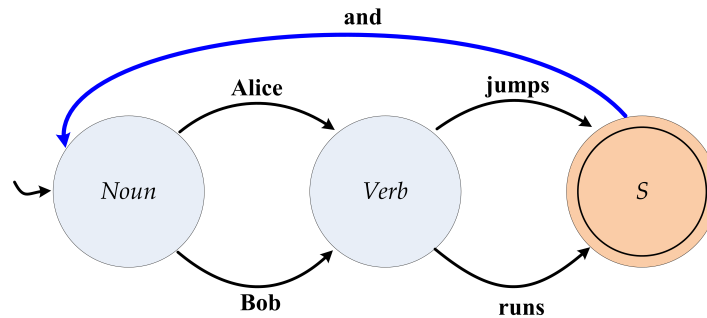
Figure 2.2. RTN with a cycle.
