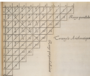
Pascal's Triangle
